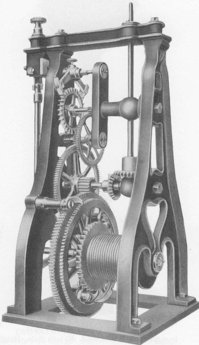
POST CLOCK MOVEMENT - 1907
